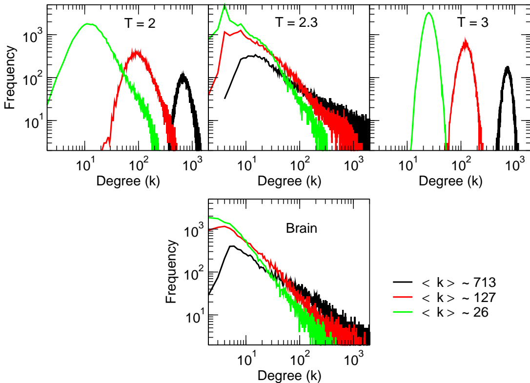
FIG. 4: Degree distribution for positively correlated networks. Top three panels depict the degree distribution for the Ising networks at T = 2 , T = 2.3 and T = 3 for three representative values of \langle k \rangle \approx 26, 127 , and 713 . Bottom panel: Degree distribution for positively correlated brain network for the same three values of \langle k \rangle .
