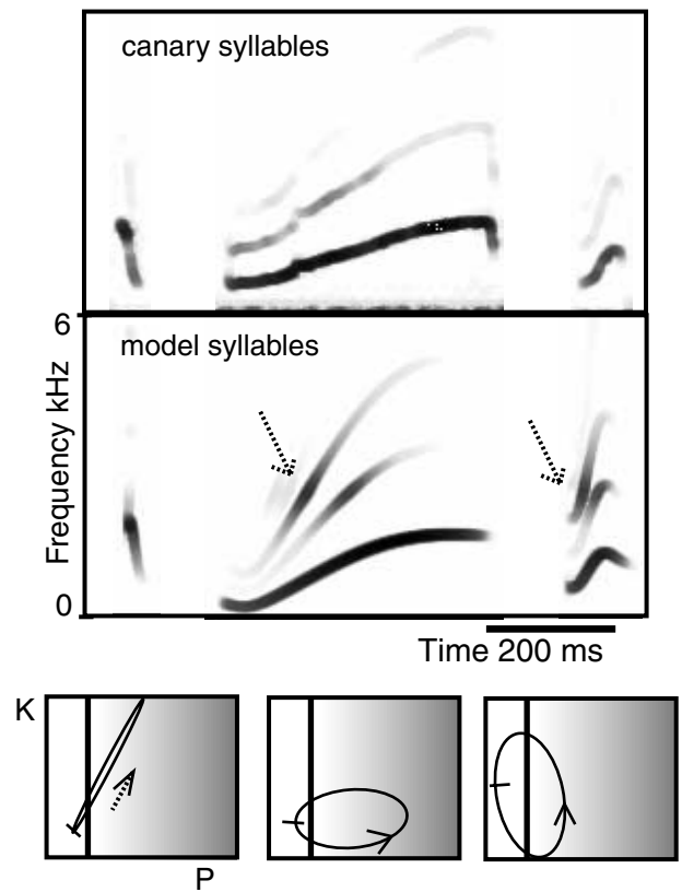
FIG. 3. Three natural syllables, three artificial syllables, and their corresponding control trajectories. The elements are illustrated in time-frequency format, which was computed through sliding, overlapped Fourier transforms. (Pixel grey level represents the power of sound on a logarithmic scale.) Parameters are drawn with respect to Fig. 2. Arrows indicate the direction of traversal over the curve. In each case, the trajectory begins at the minimum pressure value and traverse the ellipse in a counter-clockwise direction. As discussed in the text, the parametrization of time in each ellipse is chosen to cause a slowing of traversal rate near the point of maximum pressure. For each syllable, the vocal tract filter has the following parameters: L_1 = 3.0 cm, L_2 = 1.0 cm, A_1 = 0.15 cm, A_2 = 0.4 cm, and \alpha = 0.8 . This filter leads to a transient emphasis of the power of the second and third harmonics as indicated by the arrows. A further point can be illustrated with this figure. For fast syllables, sound production at a particular point P_b and K is not equivalent to the steady state sound production. Were it equivalent, syllable one would be almost symmetric in time. In effect, there is some overlap between the time scale of equilibration of the oscillation and the time scale of the fastest syllables.
