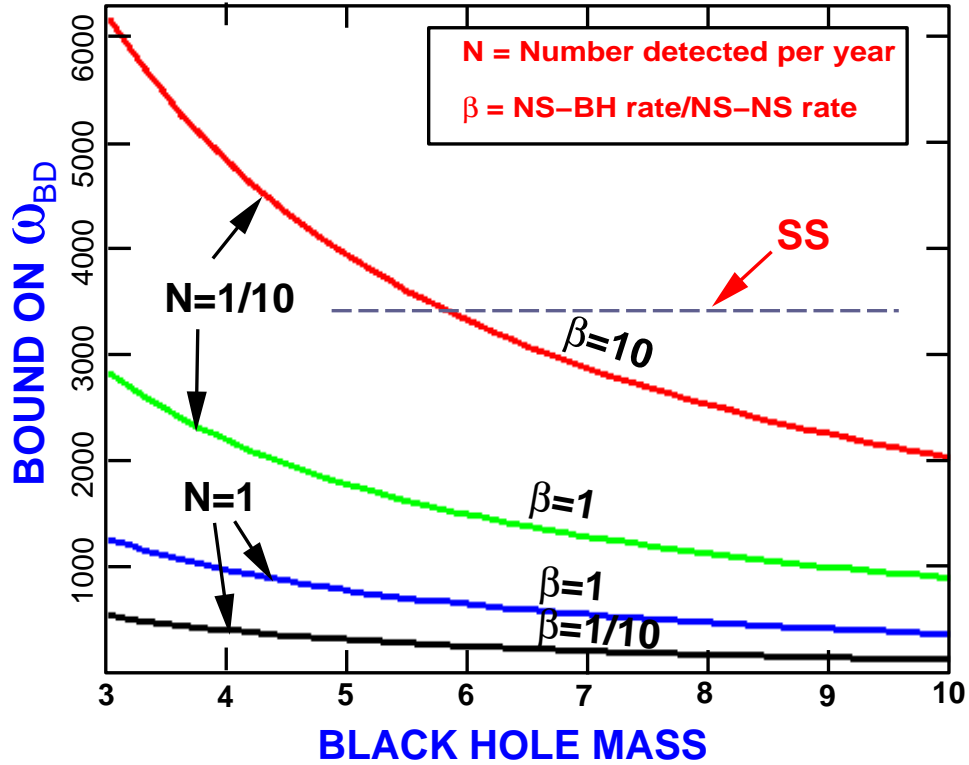
Figure 10: Bounds on the scalar-tensor coupling constant \omega_{BD} from gravitational-wave observations of inspiralling black-hole neutron-star systems. The solar system bound is around \omega_{BD} = 3500 .
