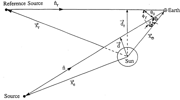
Figure 4: Geometry of light deflection measurements.
