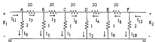
Fig. 1. Ladder network.
